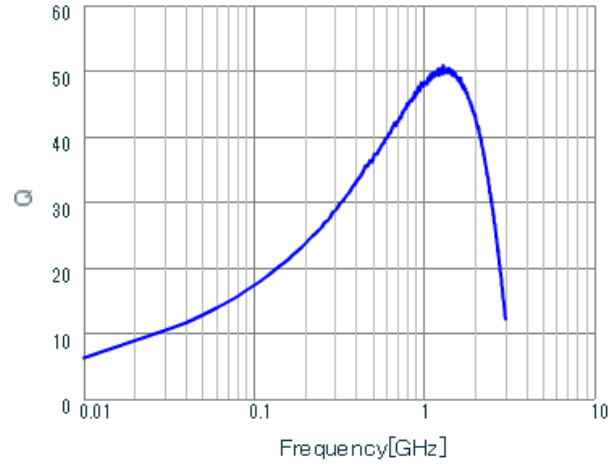
LQG15WZ15NG02 Q.
