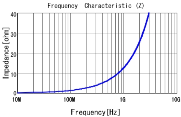
■ LQG15WZ2N0B02 |Z|
