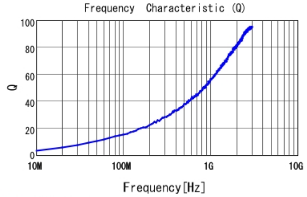
■ LQG15WZ2N0B02 Q
