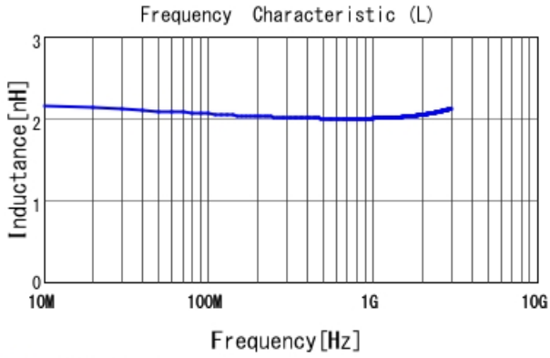
■ LQG15WZ2N0B02 L
