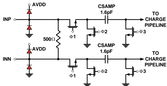
FIGURE 47. ANALOG INPUTS
